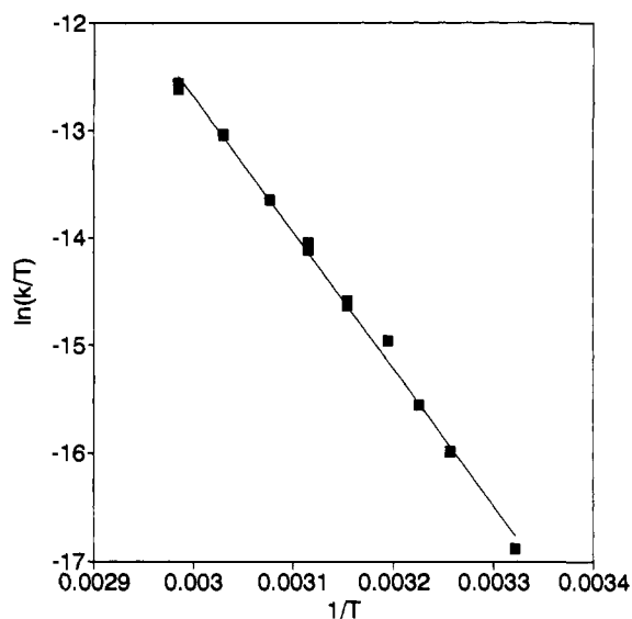
Figure 2. Eyring plot for the conversion of 3 into 2.
