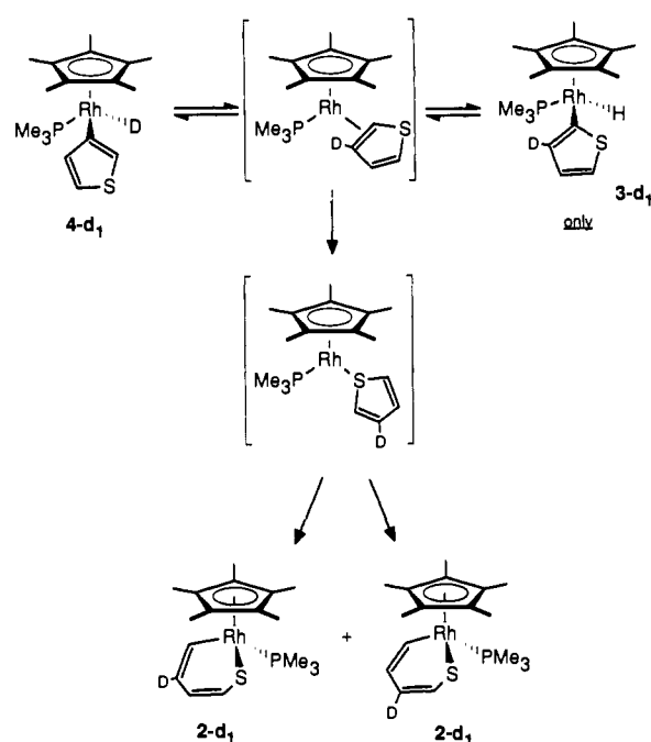
Scheme VIII. 3-Thienyl Deuteride Rearrangement Indicates that \eta^2 -Intermediate Is not Fluxional
