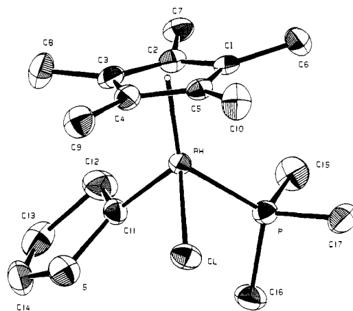
Figure 1. ORTEP drawing of (C 5 Me 5 )Rh(PMe 3 )(2-thienyl)Cl. Ellipsoids are shown at the 50% level.
